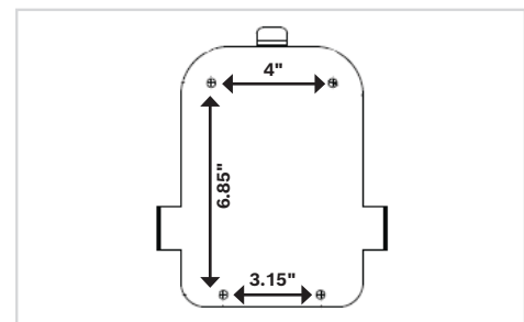
Wall-mount bracket
