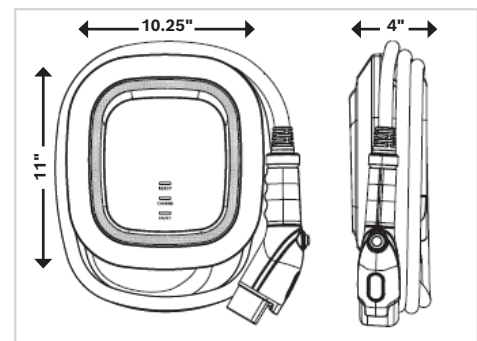
Dimensions of charger
